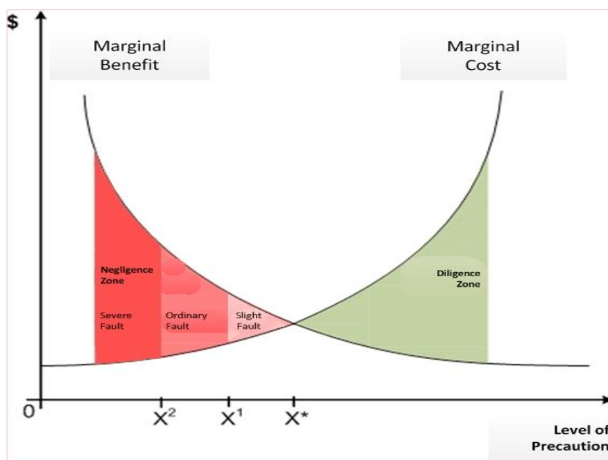
Figure 2 – Geometric representation of the incremental Learned Hand standard as criterion for negligence gradation.
