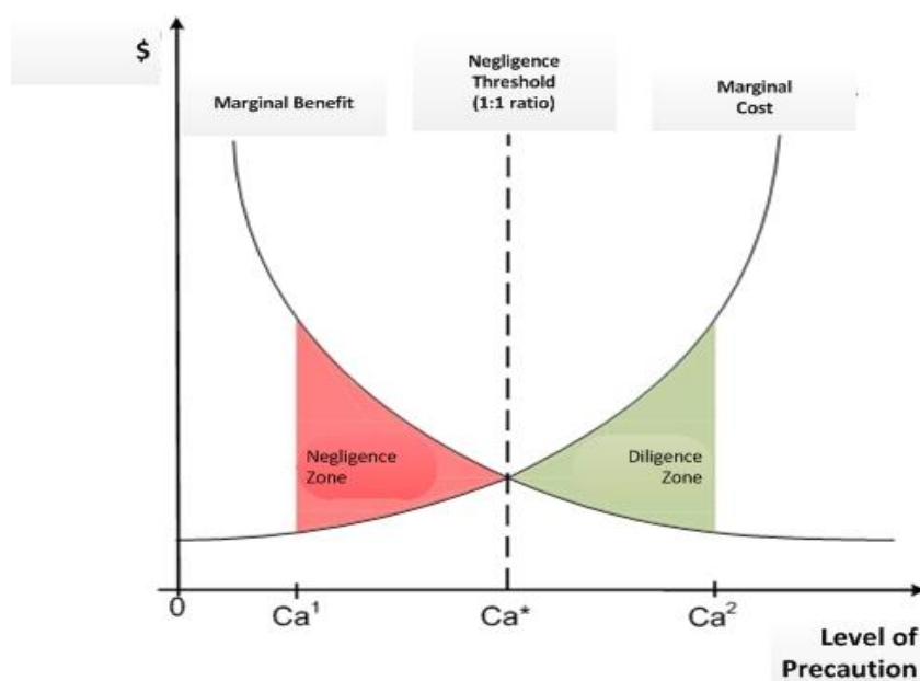
Figure 1 - Graphical representation of the incremental Learned Hand standard as criterion for negligence assessment. Adapted from Veljanovski (2006, p. 104). Level of precaution in physical units; cost of accidents in monetary units.
